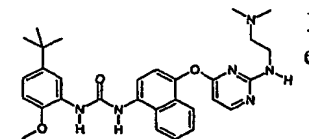
1-(5-tert-Butyl-2-methoxy-phenyl)-3-{4-[2-(2-dimethylamino-ethylamino)-pyrimidin-4-yloxy]-naphthalen-1-yl}-urea;
